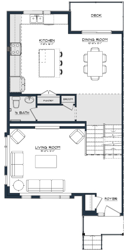
1ST FLOOR 848 sqft
