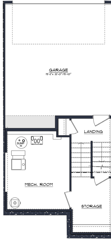
BASEMENT + GARAGE 685 sqft
